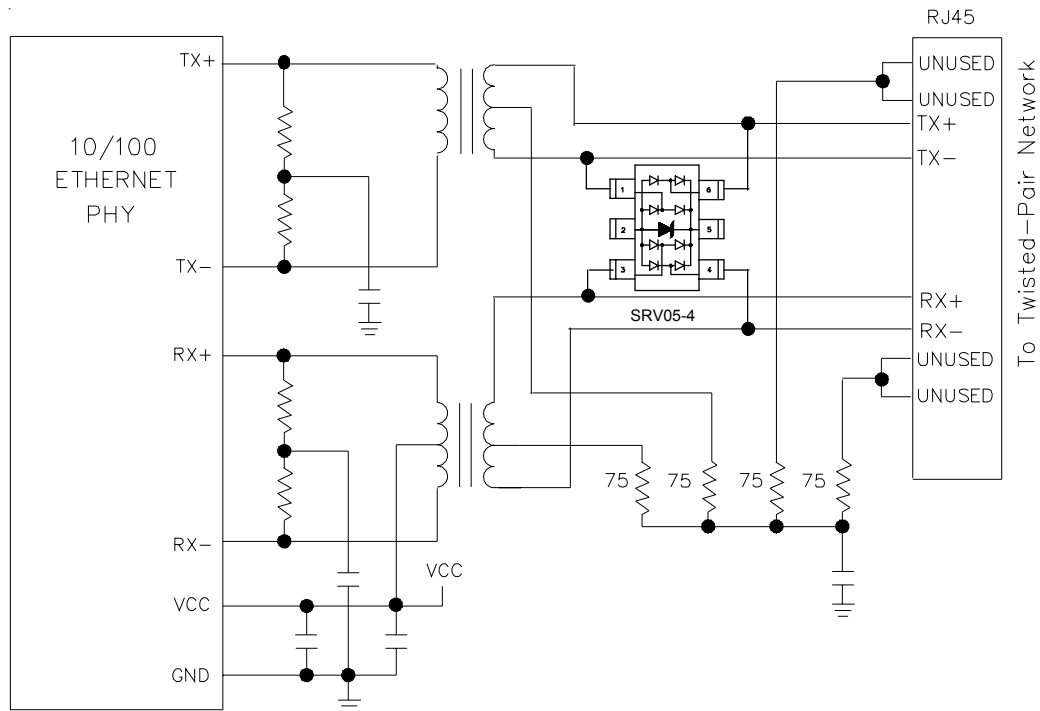
Figure 8 - 10/100 Ethernet Differential Protection
