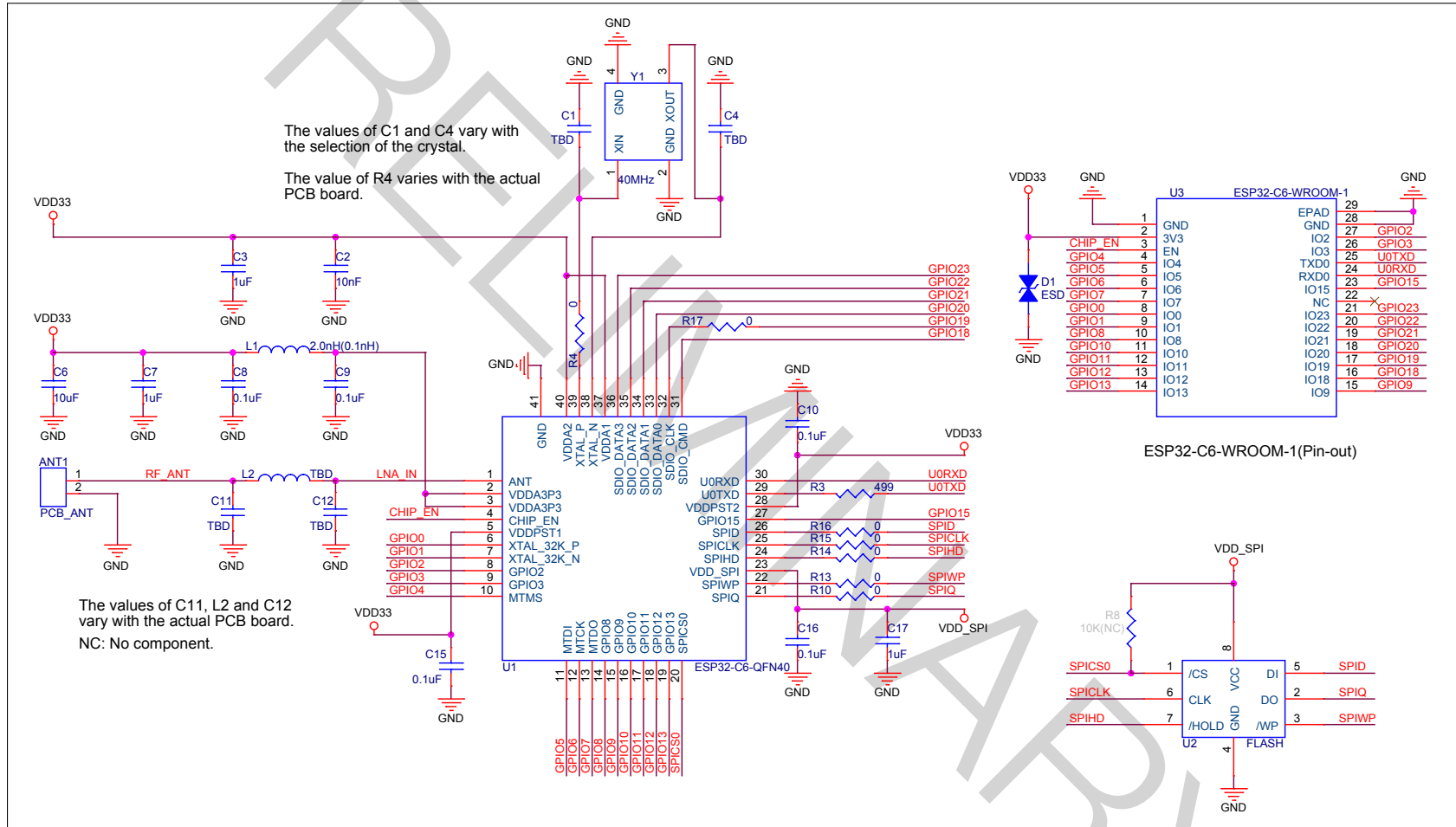
Figure 3: ESP32-C6-WROOM-1 Schematics
