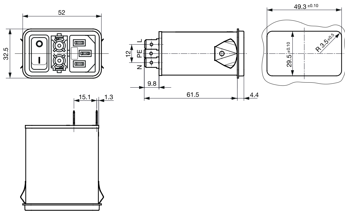
Snap-in mounting from front side
