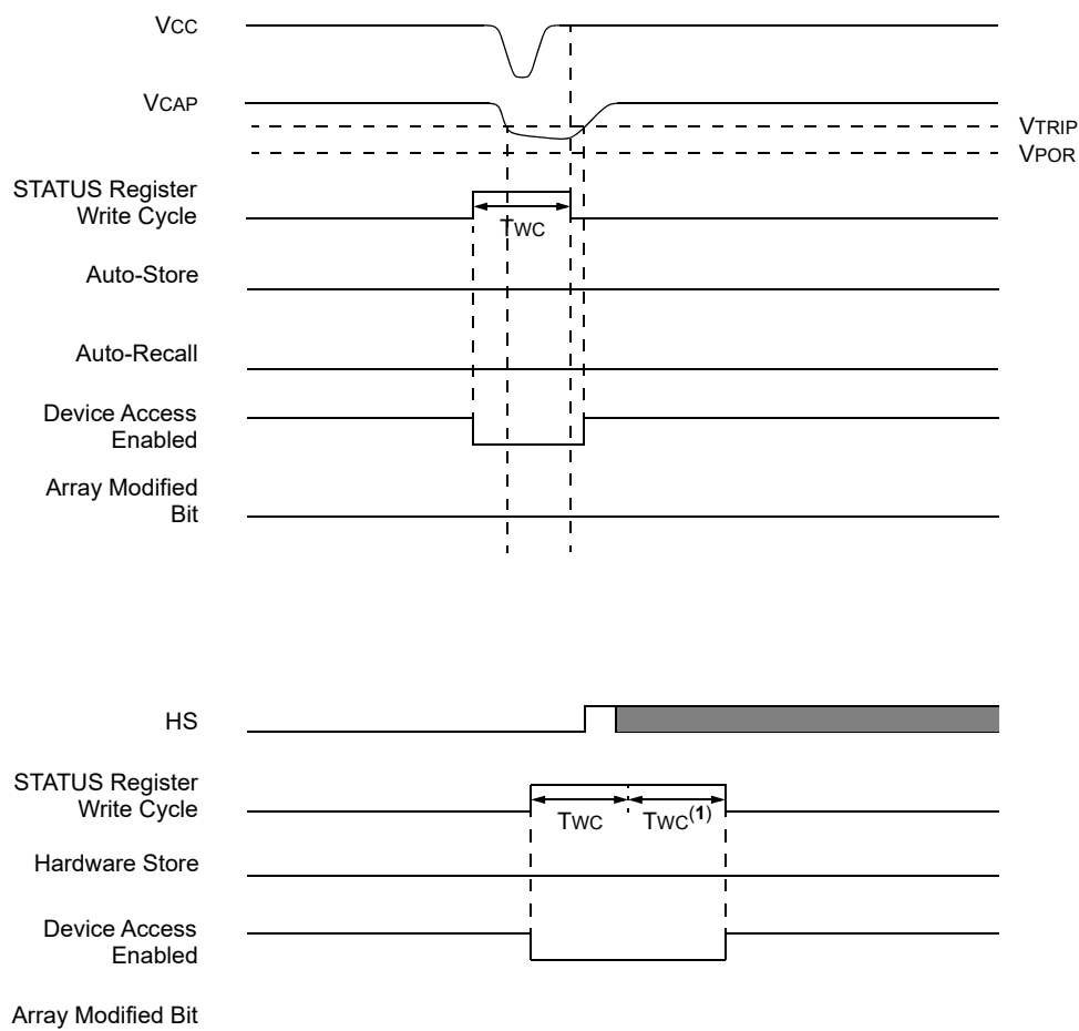
FIGURE 2-14: STORE DURING STATUS REGISTER WRITE CYCLE SCENARIOS (WITH AM = 0)
