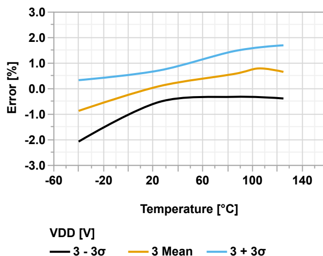
Figure 38-90. ADC0REF Voltage Error vs. Temperature ( V_{DD} = 3.0V , V_{VREF} = 1.024V )
