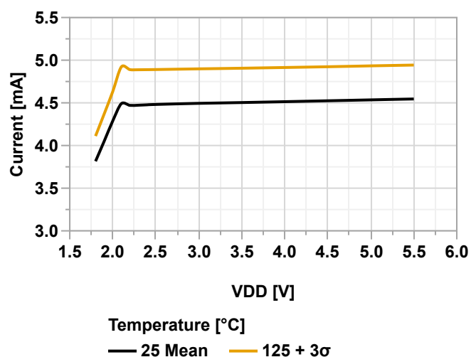
Figure 38-4. Active Power Consumption vs. V_{DD} (MCLKCTRLA.CLKSEL = OSCHF, OSCF = 24 MHz)
