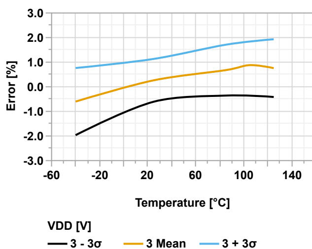
Figure 38-101. ACREF Voltage Error vs. Temperature ( V_{DD} = 3.0V , V_{VREF} = 2.5V )
