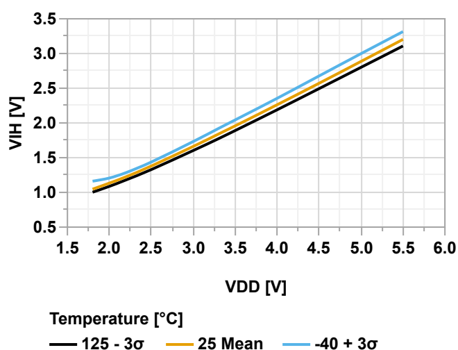
Figure 38-76. Input Pin with I 2 C Trigger - Minimum V_{IH} vs. V_{DD}
