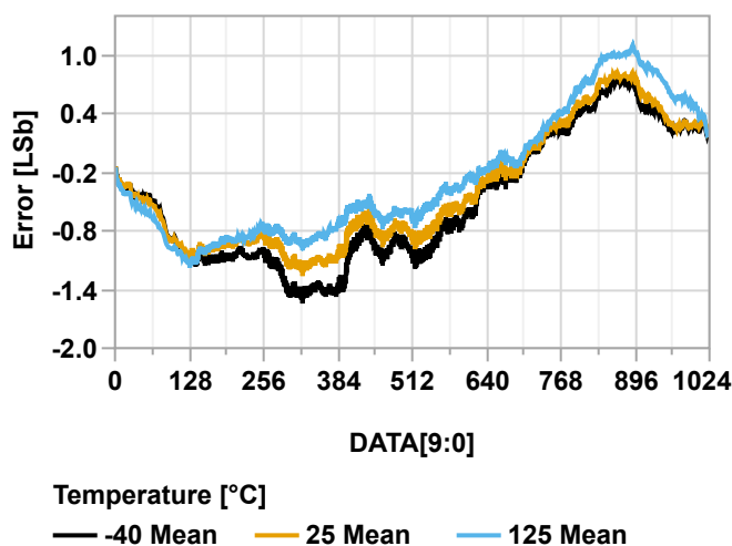
Figure 38-153. INL vs. DAC Code ( V_{\text{REFA}} = V_{\text{DD}} = 3.0\text{V} )
