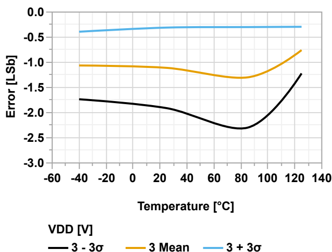
Figure 38-149. Offset Error vs. Temperature ( V_{\text{REFA}} = V_{\text{DD}} = 3.0\text{V} )
