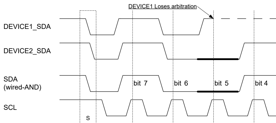
Figure 27-7. TWI Arbitration
