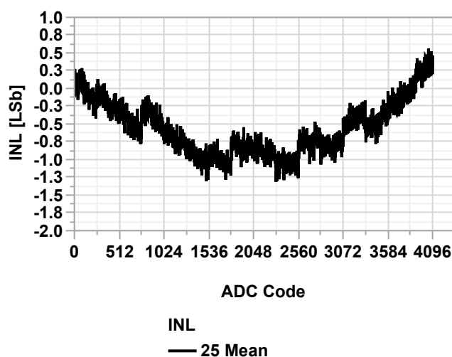
Figure 38-115. INL vs. ADC code (ADC Single Ended Mode @60 kps, V_{\text{DD}} = 3.0\text{V} )
