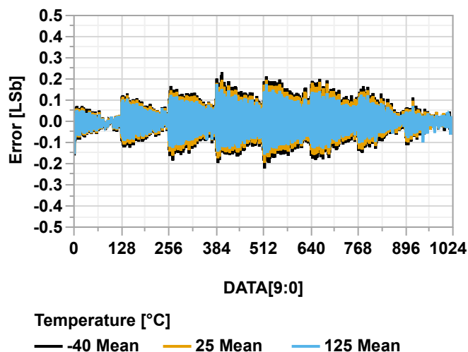
Figure 38-154. INL vs. DAC Code ( V_{\text{REFA}} = V_{\text{DD}} = 5.5\text{V} )
