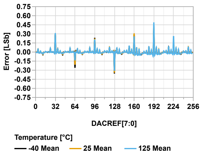
Figure 38-161. INL vs. DAC Code ( V_{\text{REFA}} = V_{\text{DD}} = 3.0\text{V} )
