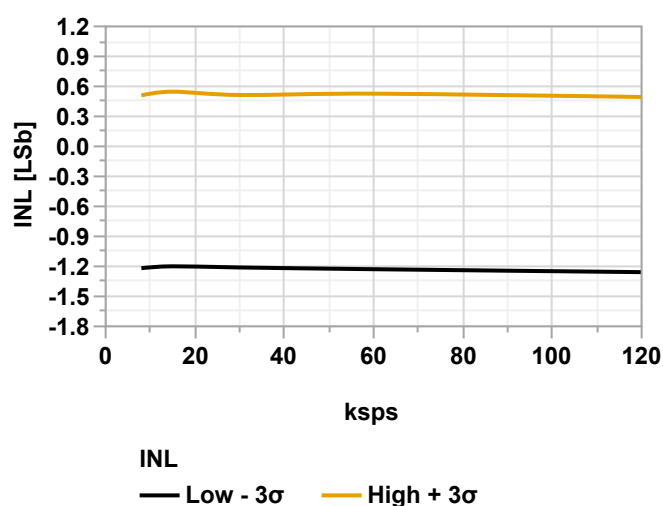
Figure 38-119. INL vs. Sample Rate (ADC Single Ended Mode, V_{\text{REFA}} = V_{\text{DD}} = 3.0\text{V} , T = 125^\circ\text{C} )
