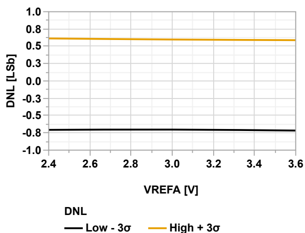
Figure 38-127. DNL vs. V_{\text{REFA}} (ADC Differential Mode @60 kps, V_{\text{DD}} = 3.6\text{V} , T = 25^\circ\text{C} )
