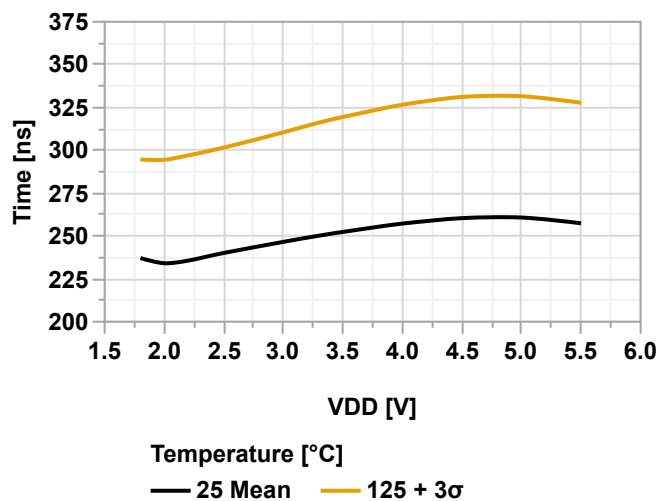
Figure 38-138. Rising Edge Response Time vs. V_{DD} ( V_{CM} = V_{DD}/2 , CTRLA.POWER = 0x01)
