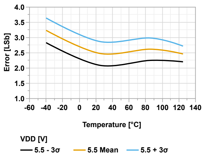
Figure 38-150. Offset Error vs. Temperature ( V_{\text{REFA}} = V_{\text{DD}} = 5.5\text{V} )
