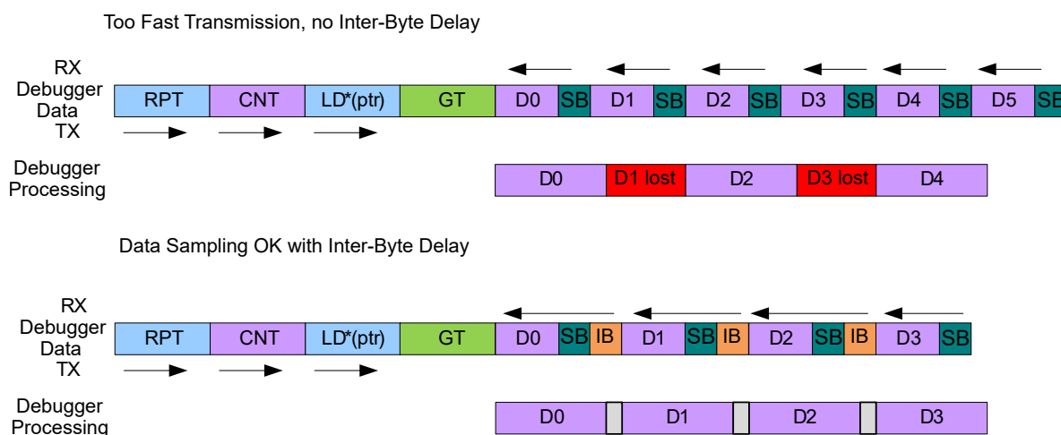
Figure 35-17. Inter-Byte Delay Example with LD and RPT
