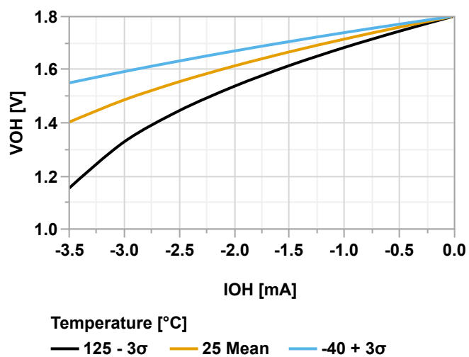
Figure 38-83. Output Pin - Minimum V_{OH} vs. Current, V_{DD} = 1.8\text{V}
