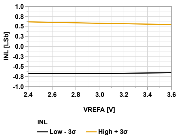
Figure 38-132. INL vs. V_{\text{REFA}} (ADC Differential Mode @60 kps, V_{\text{DD}} = 3.6\text{V} , T = 85^\circ\text{C} )
