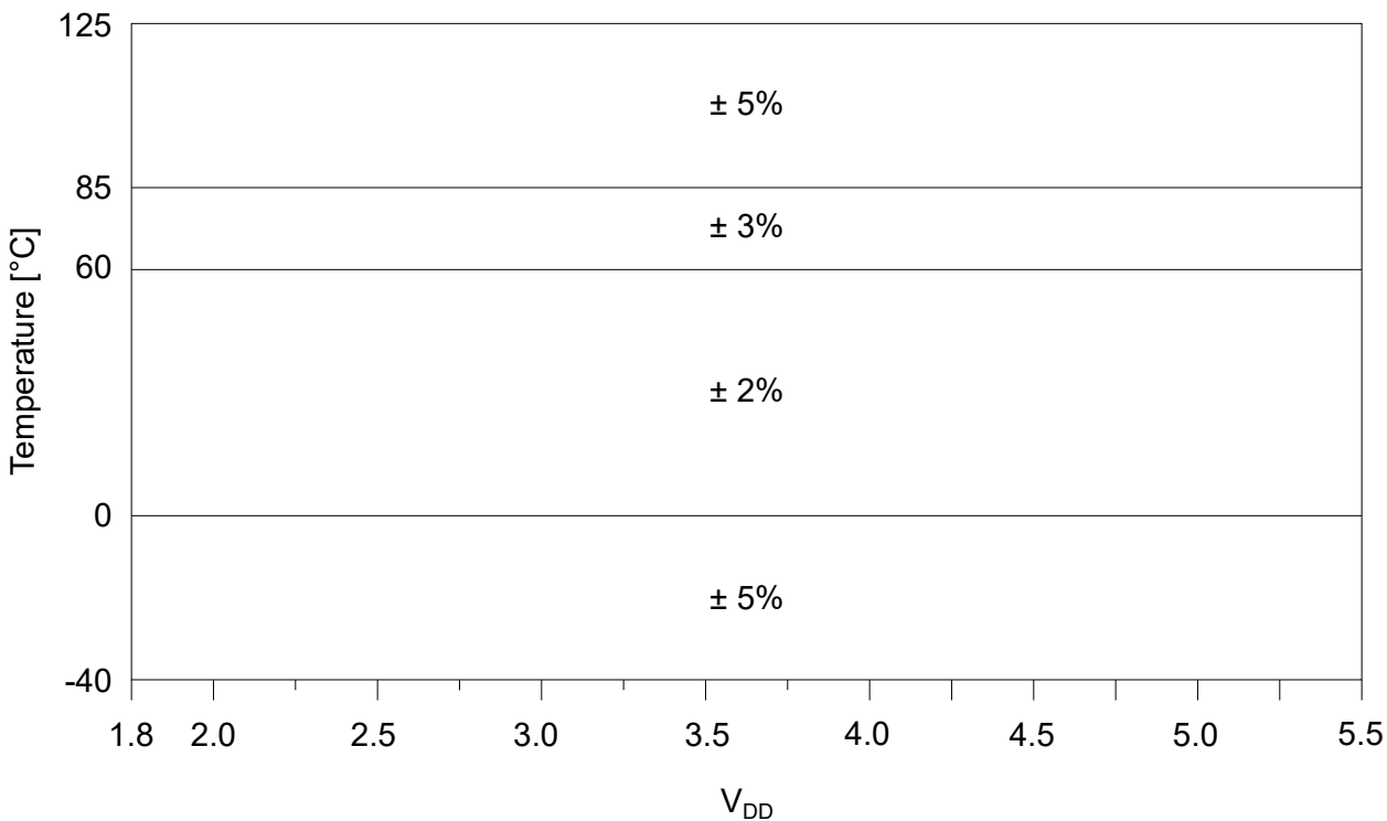
Figure 37-2. Precision Calibrated OSCHF (4 MHz) Frequency Accuracy Over Device V_{DD} and Temperature
