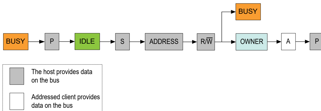
Figure 27-8. Quick Command Frame Format
