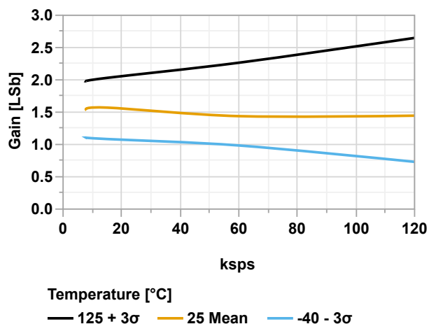
Figure 38-123. Negative Gain Error vs. Sample Rate (ADC Differential Mode, V_{\text{REFA}} = V_{\text{DD}} = 3.6\text{V} )
