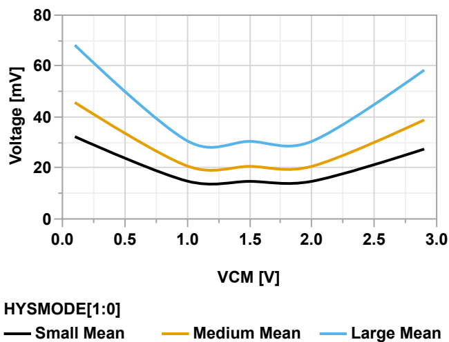
Figure 38-146. Input Hysteresis vs. Common Mode Voltage ( V_{DD} = 5.5V )
