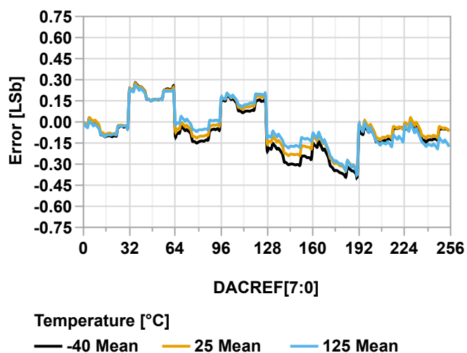
Figure 38-162. INL vs. DAC Code ( V_{\text{REFA}} = V_{\text{DD}} = 5.5\text{V} )
