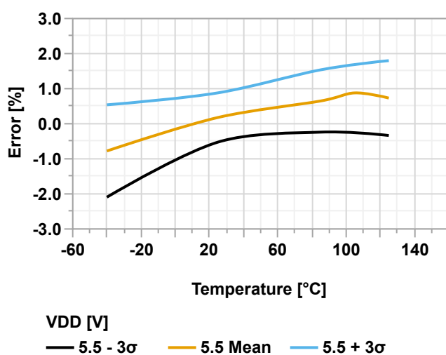
Figure 38-93. ADC0REF Voltage Error vs. Temperature ( V_{DD} = 5.5V , V_{VREF} = 2.5V )
