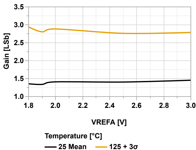
Figure 38-110. Gain Error vs. V_{REFA} (ADC Single Ended Mode @60 kps, V_{DD} = 3.0V )
