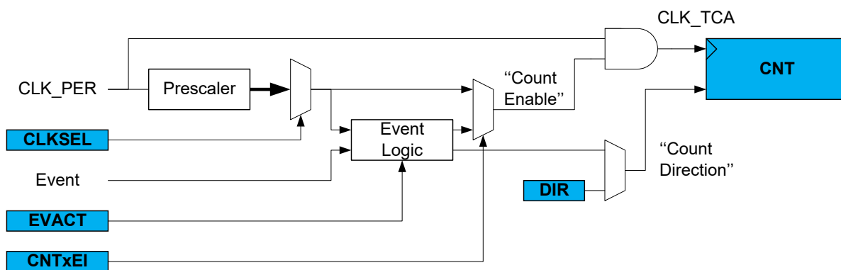
Figure 21-3. Timer/Counter Clock Logic
