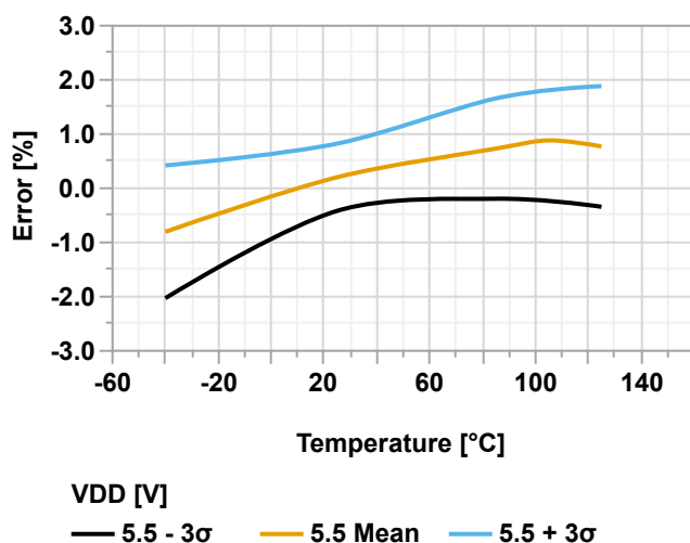
Figure 38-89. ADC0REF Voltage Error vs. Temperature ( V_{DD} = 5.5V , V_{VREF} = 1.024V )
