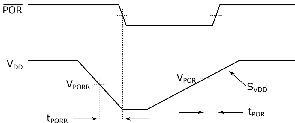
Figure 37-1. \overline{POR} and \overline{POR} Re-Arm with Slow Rising V_{DD}
