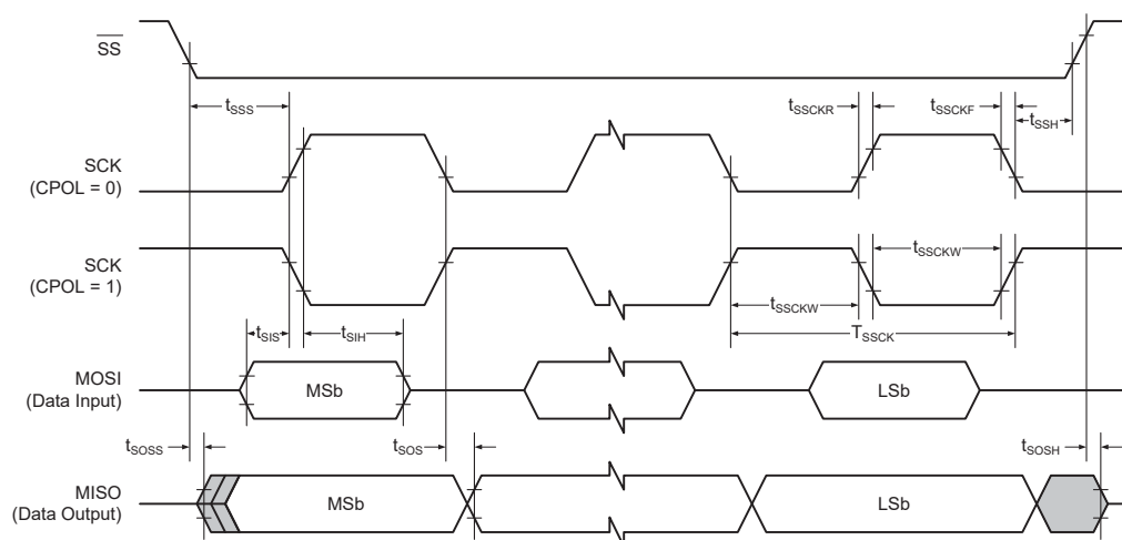
Figure 37-6. SPI - Timing Requirements in Client Mode
