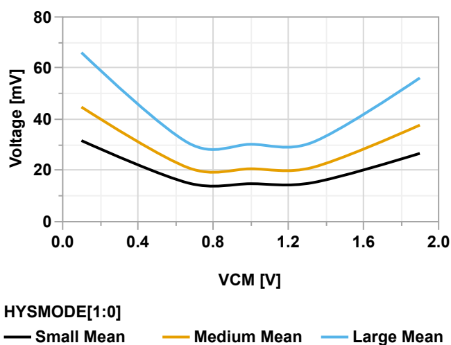
Figure 38-142. Input Hysteresis vs. Common Mode Voltage ( V_{DD} = 2.0V )
