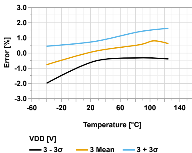
Figure 38-94. ADC0REF Voltage Error vs. Temperature ( V_{DD} = 3.0V , V_{VREF} = 2.5V )
