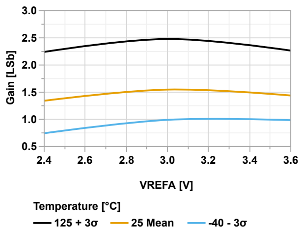
Figure 38-122. Negative Gain Error vs. V_{\text{REFA}} (ADC Differential Mode @60 kps, V_{\text{DD}} = 3.6\text{V} )
