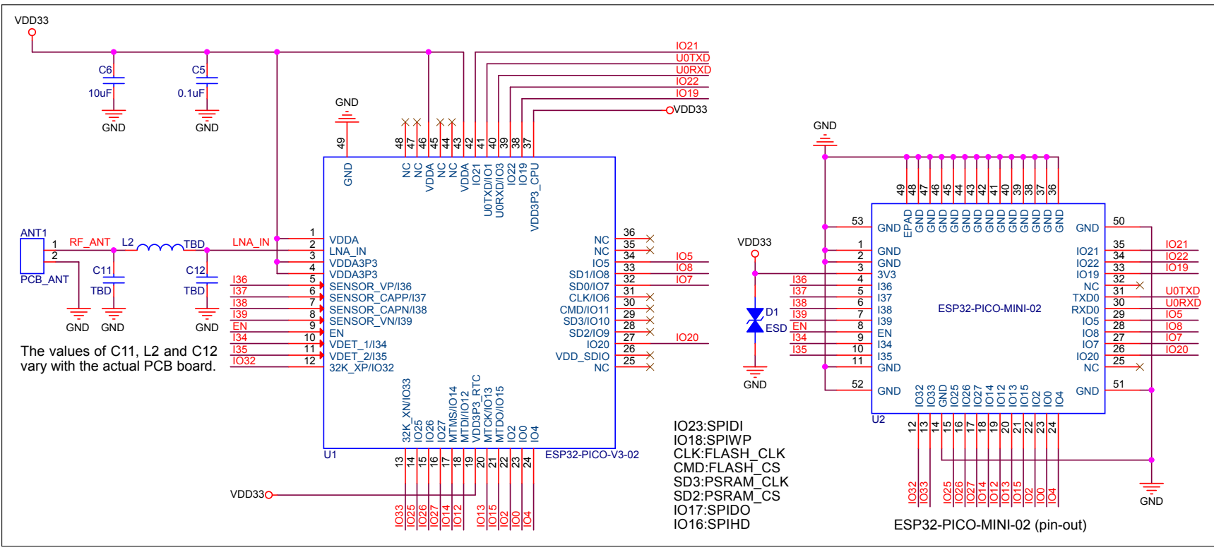
Figure 5: ESP32-PICO-MINI-02 Schematics
