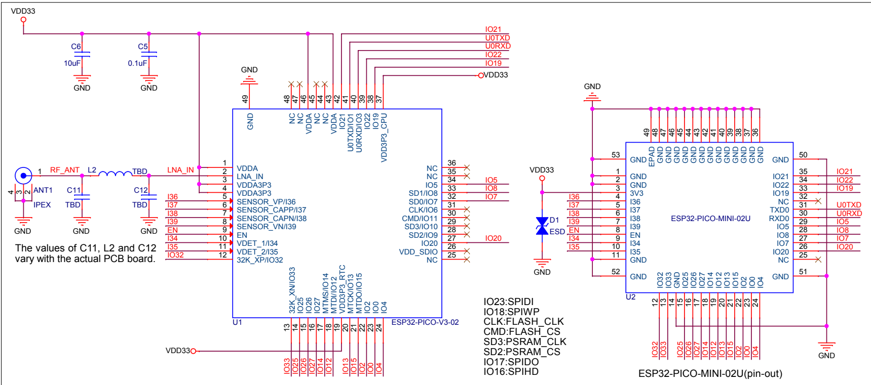
Figure 6: ESP32-PICO-MINI-02U Schematics
