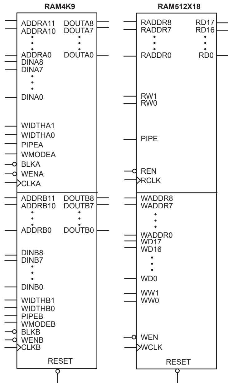
FIGURE 2-30: RAM MODELS
