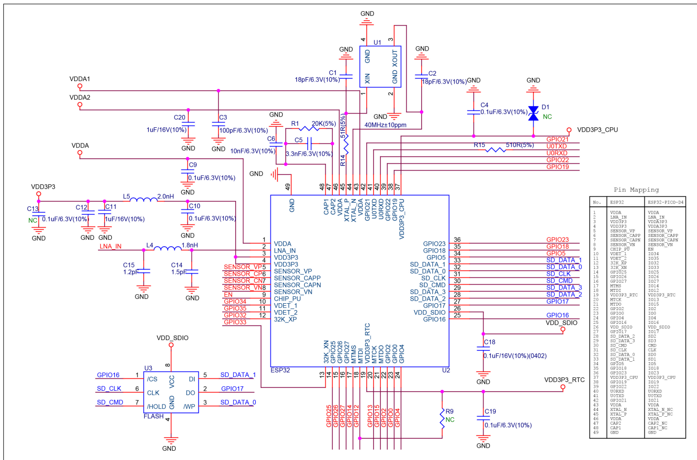
Figure 7: ESP32-PICO-D4 Schematics
