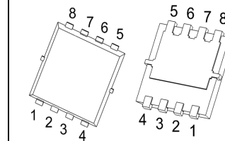
PDFNWB3.3×3.3-8L
