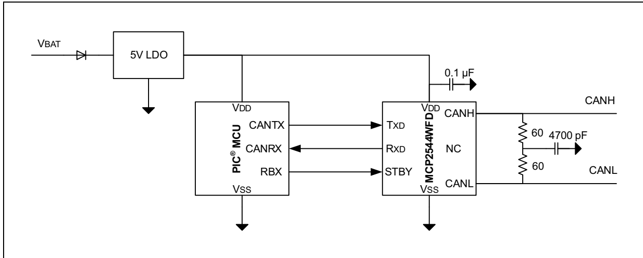
FIGURE 1-3: MCP2544WFDT WITH NC AND SPLIT TERMINATION
