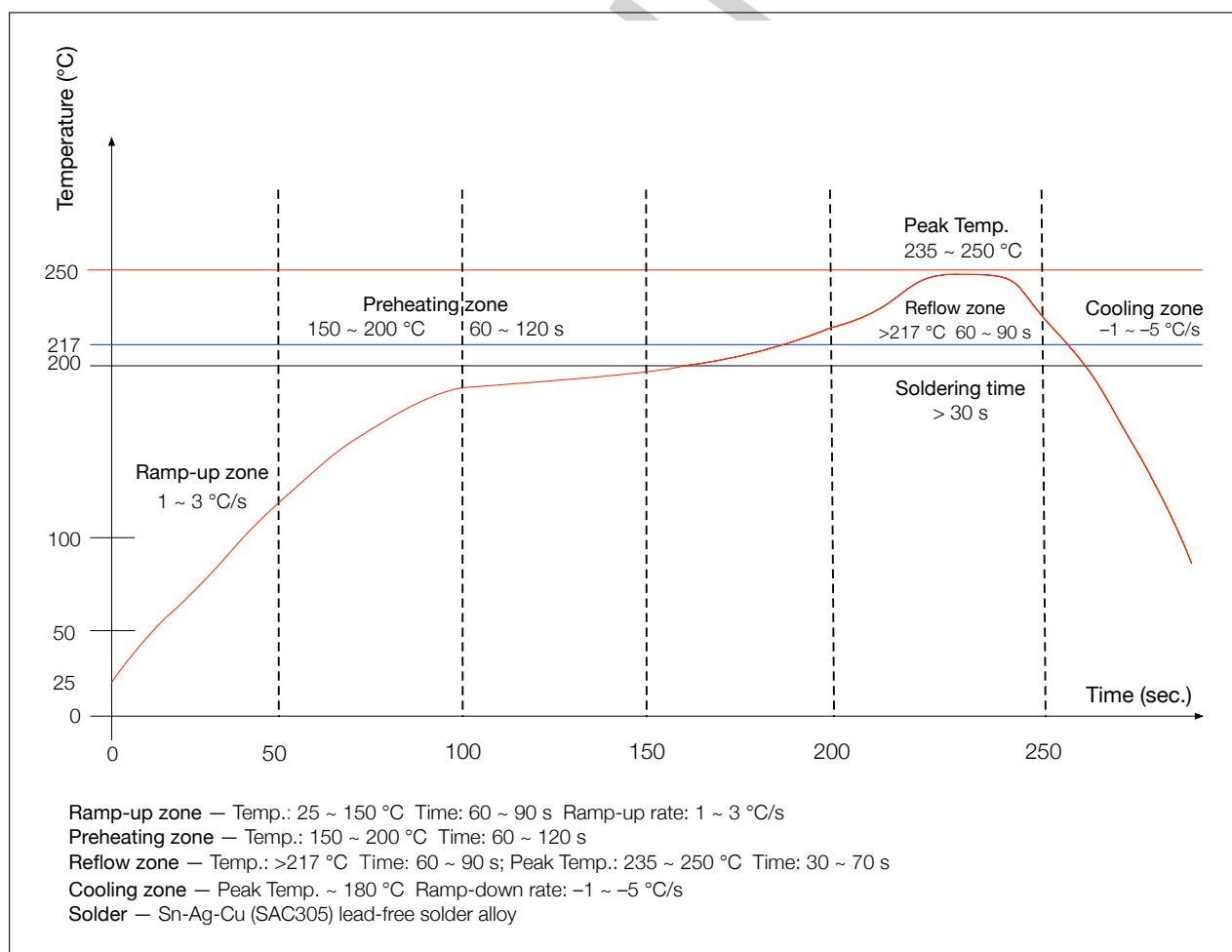
Figure 12: Reflow Profile
