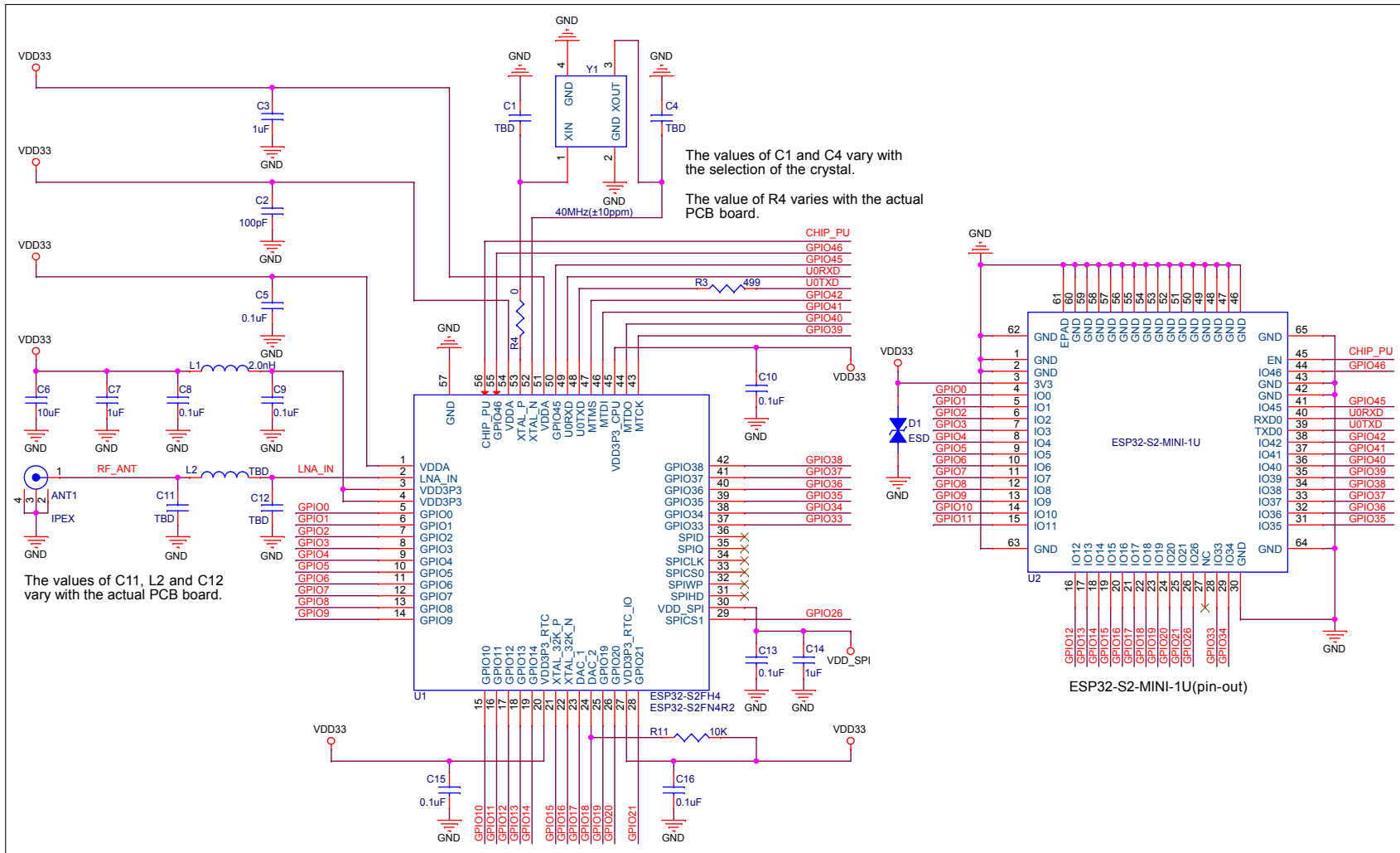
Figure 6: ESP32-S2-MINI-1U Schematics
