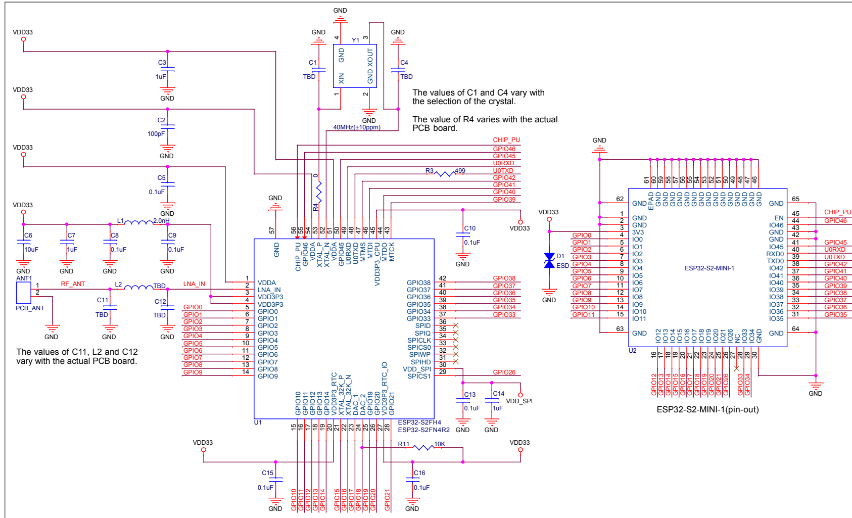
Figure 5: ESP32-S2-MINI-1 Schematics
