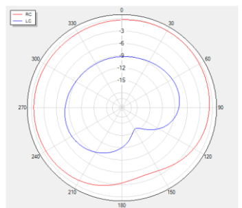
Theta=90 freq=1561MHz
