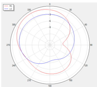
Theta=90 freq=1176MHz
