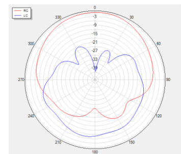
Phi=90 freq=1561MHz
