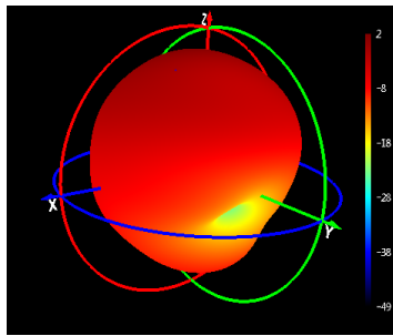
Phi=90 freq=1176MHz
