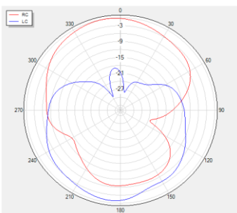
Phi=90 freq=1176MHz
