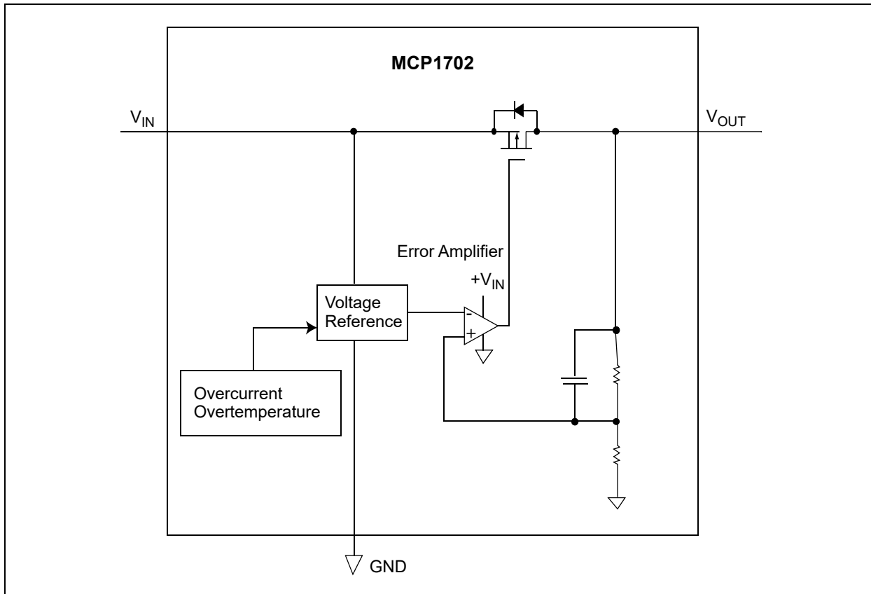
FIGURE 4-1: Block Diagram.
