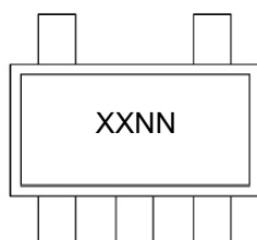
5-Lead SOT-23
