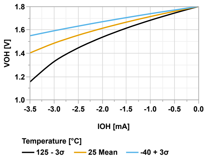
Figure 38-83. Output Pin - Minimum V_{OH} vs. Current, V_{DD} = 1.8V
