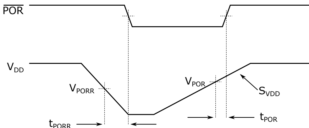
Figure 37-1. \overline{POR} and \overline{POR} Re-Arm with Slow Rising V_{DD}
