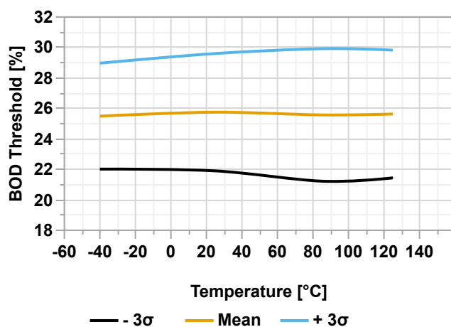
Figure 38-67. VLM Threshold vs. Temperature (VLMCTRL.VLMVLV = 0x03)
