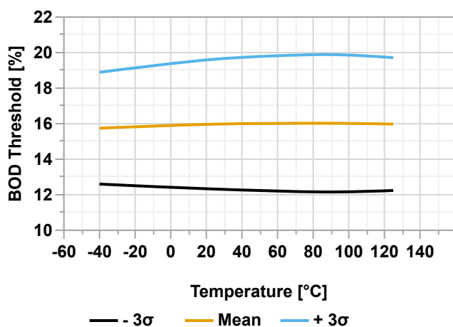
Figure 38-66. VLM Threshold vs. Temperature (VLMCTRL.VLMVLV = 0x02)
