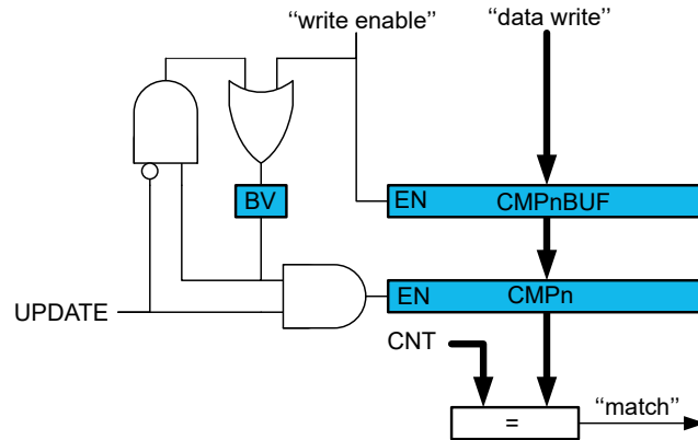
Figure 21-5. Period and Compare Double Buffering
