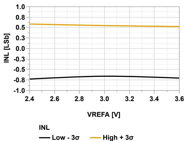
Figure 38-133. INL vs. V_{REFA} (ADC Differential Mode @60 kps, V_{DD} = 3.6V , T = 125^{\circ}C )
