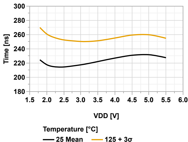
Figure 38-137. Falling Edge Response Time vs. V_{DD} ( V_{CM} = V_{DD}/2 , CTRLA.POWER = 0x01)
