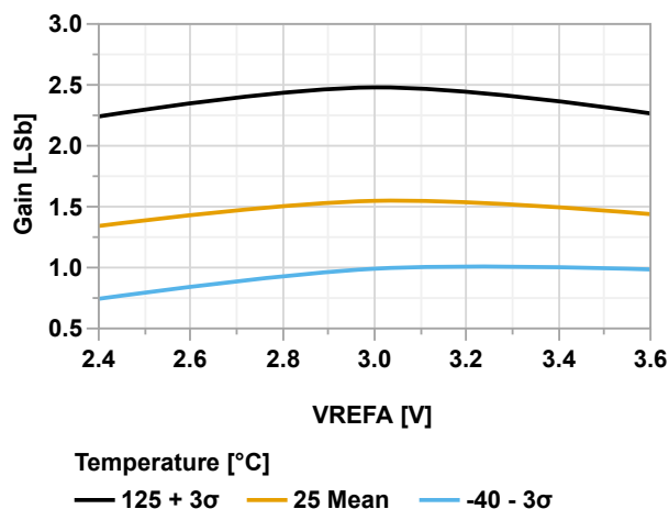
Figure 38-122. Negative Gain Error vs. V_{\text{REFA}} (ADC Differential Mode @60 kps, V_{\text{DD}} = 3.6\text{V} )
