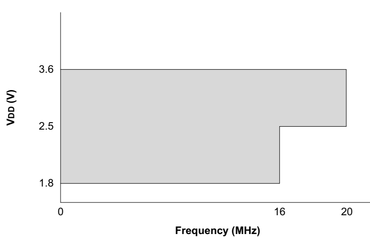
FIGURE 27-2: VOLTAGE FREQUENCY GRAPH, -40^{\circ}\text{C} \leq T_A \leq +125^{\circ}\text{C} , PIC12LF1501 ONLY
