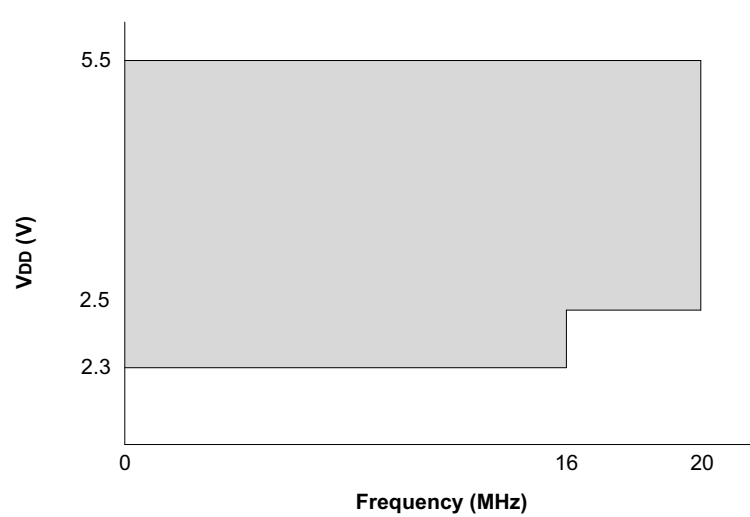
FIGURE 27-1: VOLTAGE FREQUENCY GRAPH, -40^{\circ}\text{C} \leq T_A \leq +125^{\circ}\text{C} , PIC12F1501 ONLY
