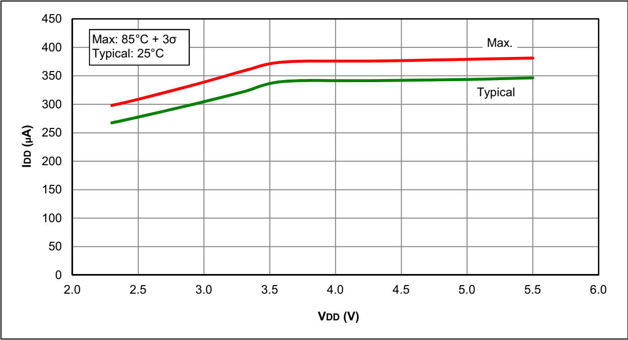
FIGURE 28-16: I_{DD} , MFINTOSC, F_{osc} = 500\text{ kHz} , PIC12F1501 ONLY
