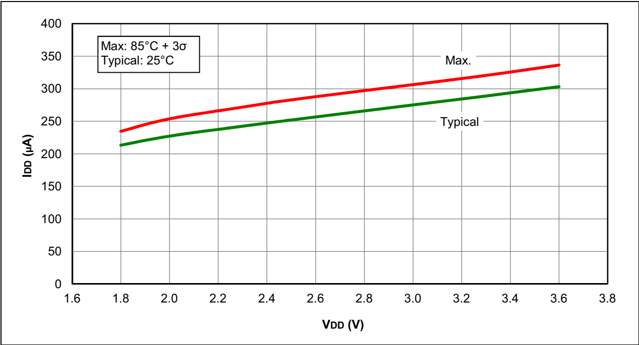
FIGURE 28-15: I_{DD} , MFINTOSC, F_{osc} = 500\text{ kHz} , PIC12LF1501 ONLY
