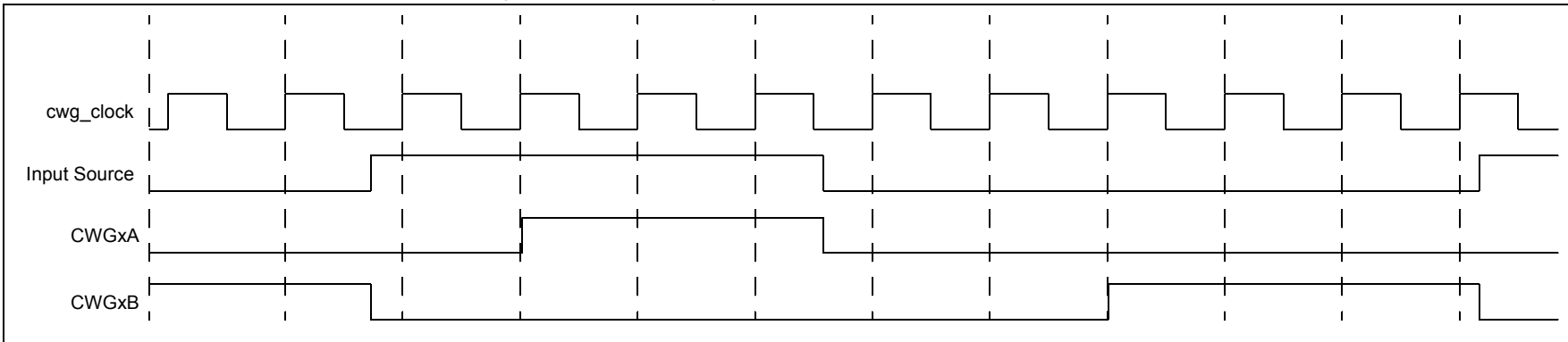
FIGURE 24-3: DEAD-BAND OPERATION, CWGxDBR = 01H, CWGxDBF = 02H
