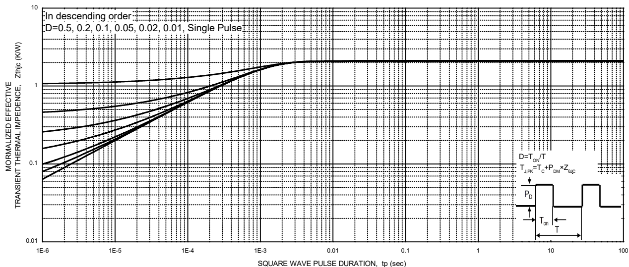
NORMALIZED TYPICAL TRANSIENT THERMAL IMPEDANCE
