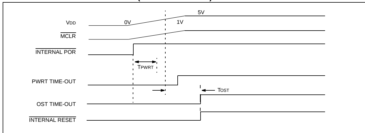
FIGURE 11-8: SLOW RISE TIME (MCLR TIED TO V DD )
