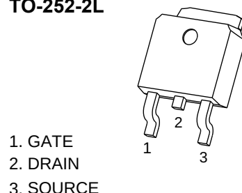
TO-252-2L
