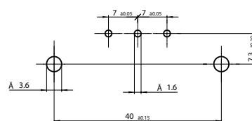
Drilling diagram for printed circuit board
