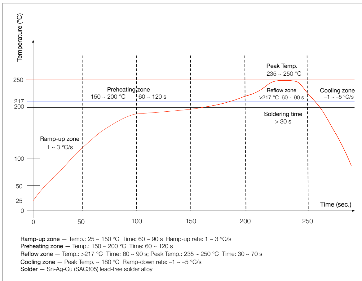
Figure 12: Reflow Profile
