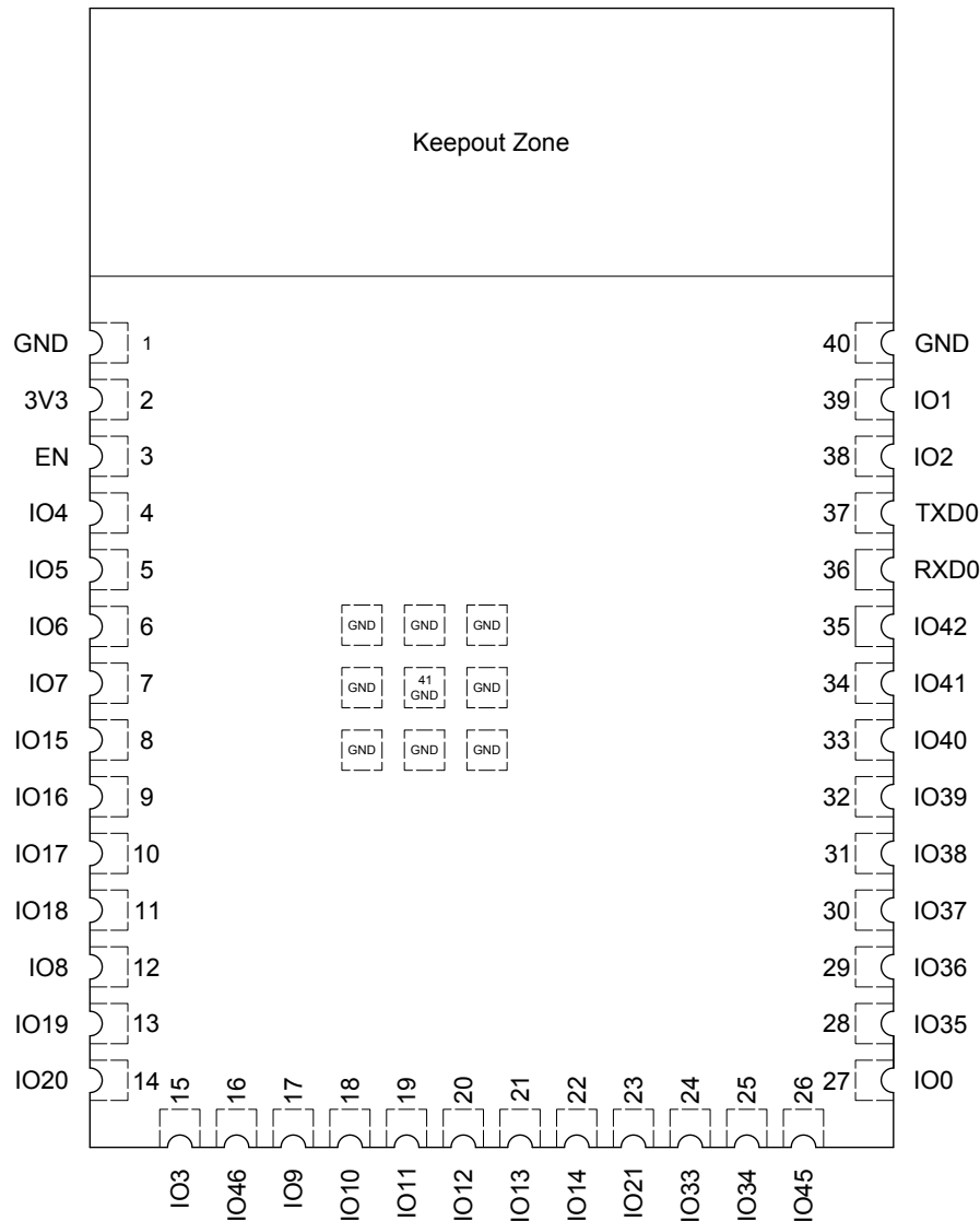
Figure 3: Module Pin Layout (Top View)
