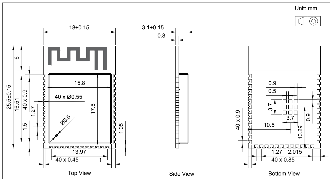
Figure 7: ESP32-S2-SOLO Physical Dimensions
