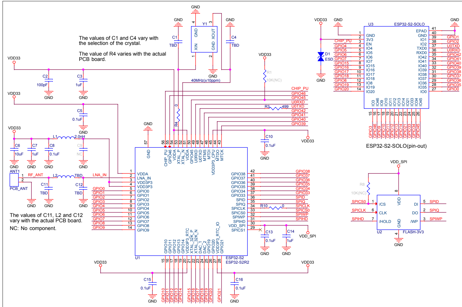
Figure 4: ESP32-S2-SOLO Schematics
