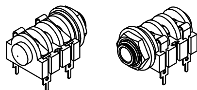
ISO VIEW
