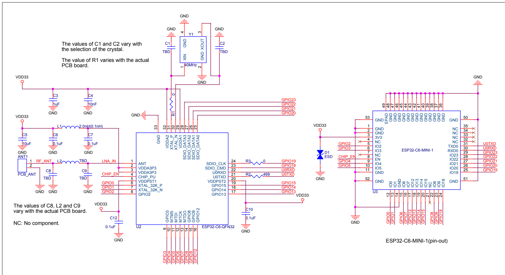
Figure 5: ESP32-C6-MINI-1 Schematics
