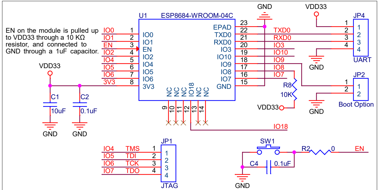
Figure 5: Peripheral Schematics
