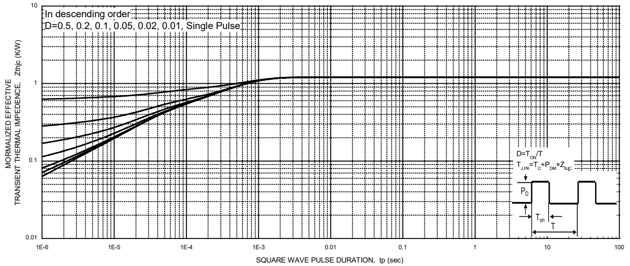
NORMALIZED TYPICAL TRAISIENT THERMAL IMPENDANCE
