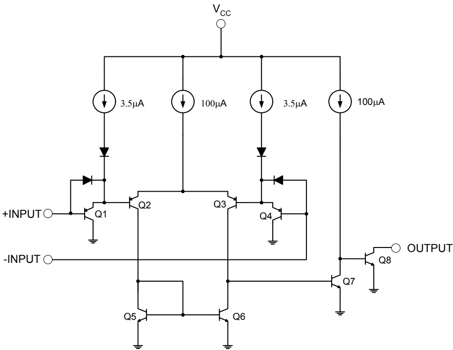
Figure 3. Functional Block Diagram of LM339 (Each Comparator)
