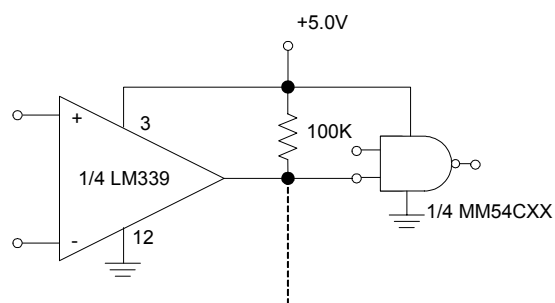
Figure 10. Driving CMOS/TTL
