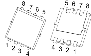
PDFNWB3.3×3.3-8L
