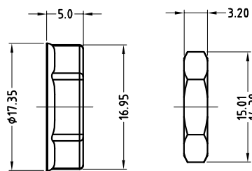
PLASTIC NUT
