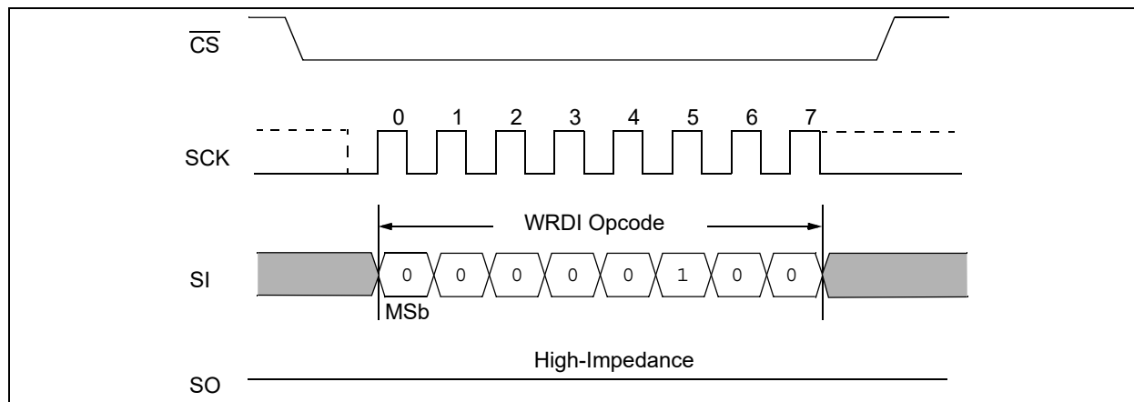
FIGURE 5-2: WRDI WAVEFORM
