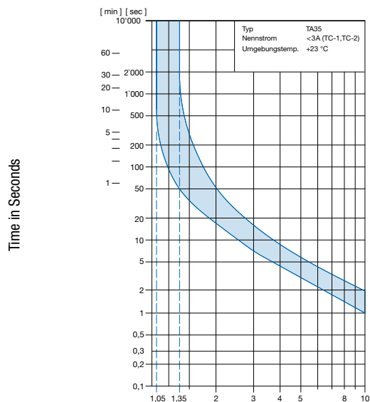
Tripping Characteristics thermal I_n < 3\text{ A}
