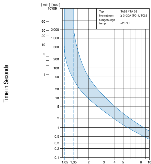
Tripping Characteristics thermal I_n \geq 3 \dots \leq 20\text{ A}
