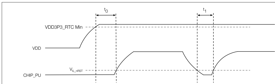
Figure 4: ESP32 Power-up and Reset Timing
