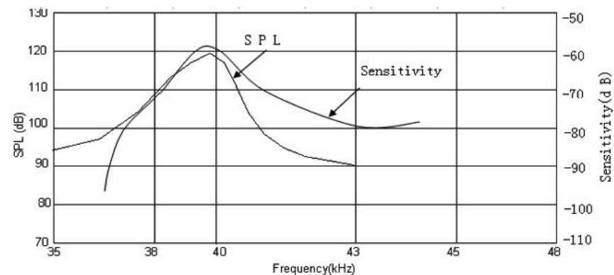
Frequency Characteristics
