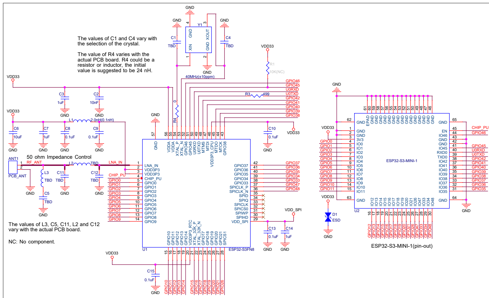
Figure 5: ESP32-S3-MINI-1 Schematics
