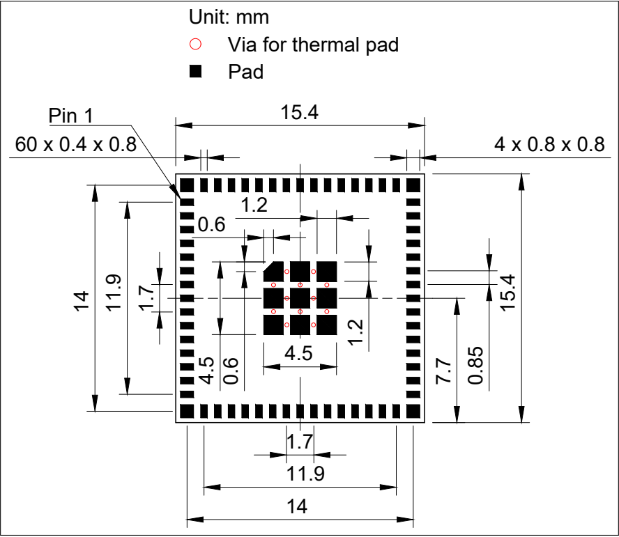
Figure 11: ESP32-S2-MINI-1U Recommended PCB Land Pattern
