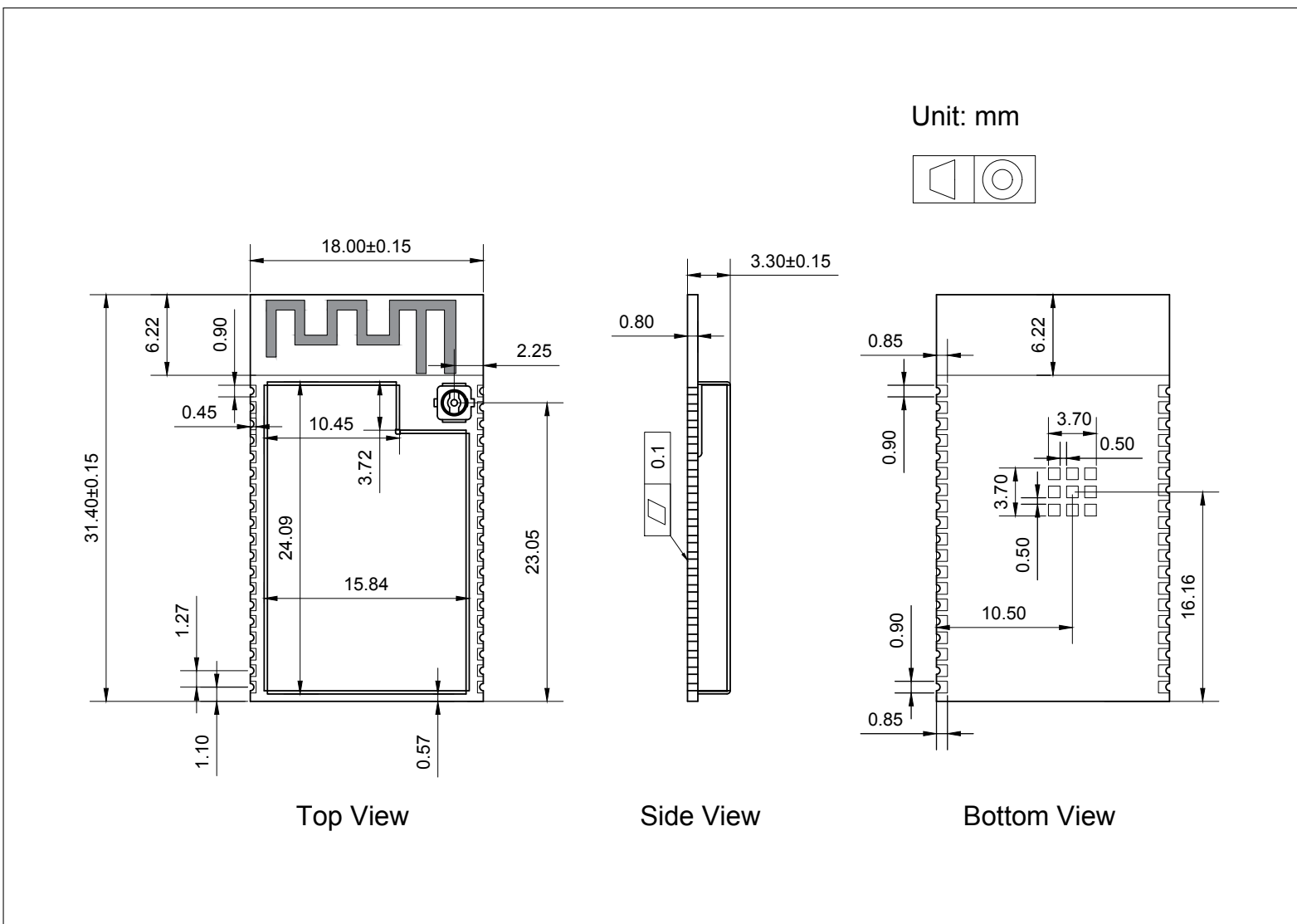
Figure 8: Physical Dimensions
