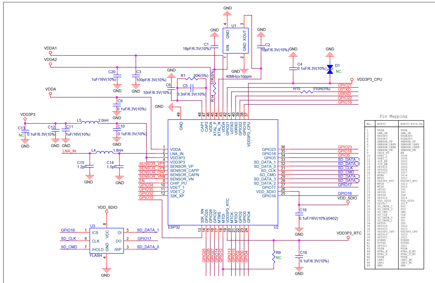
Figure 6: ESP32-PICO-D4 Schematics
