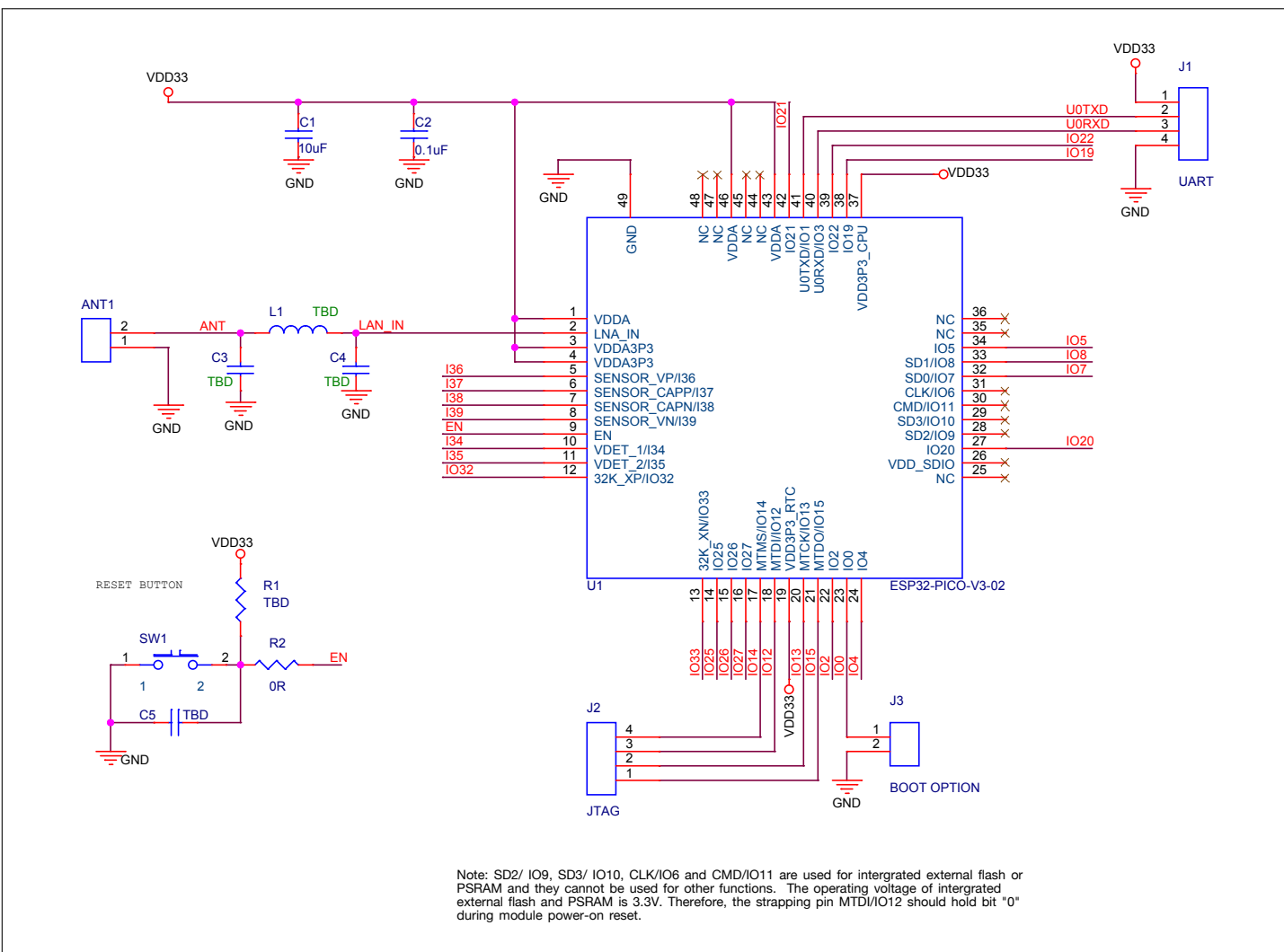
Figure 11: ESP32-PICO-V3-02 Peripheral Schematics
