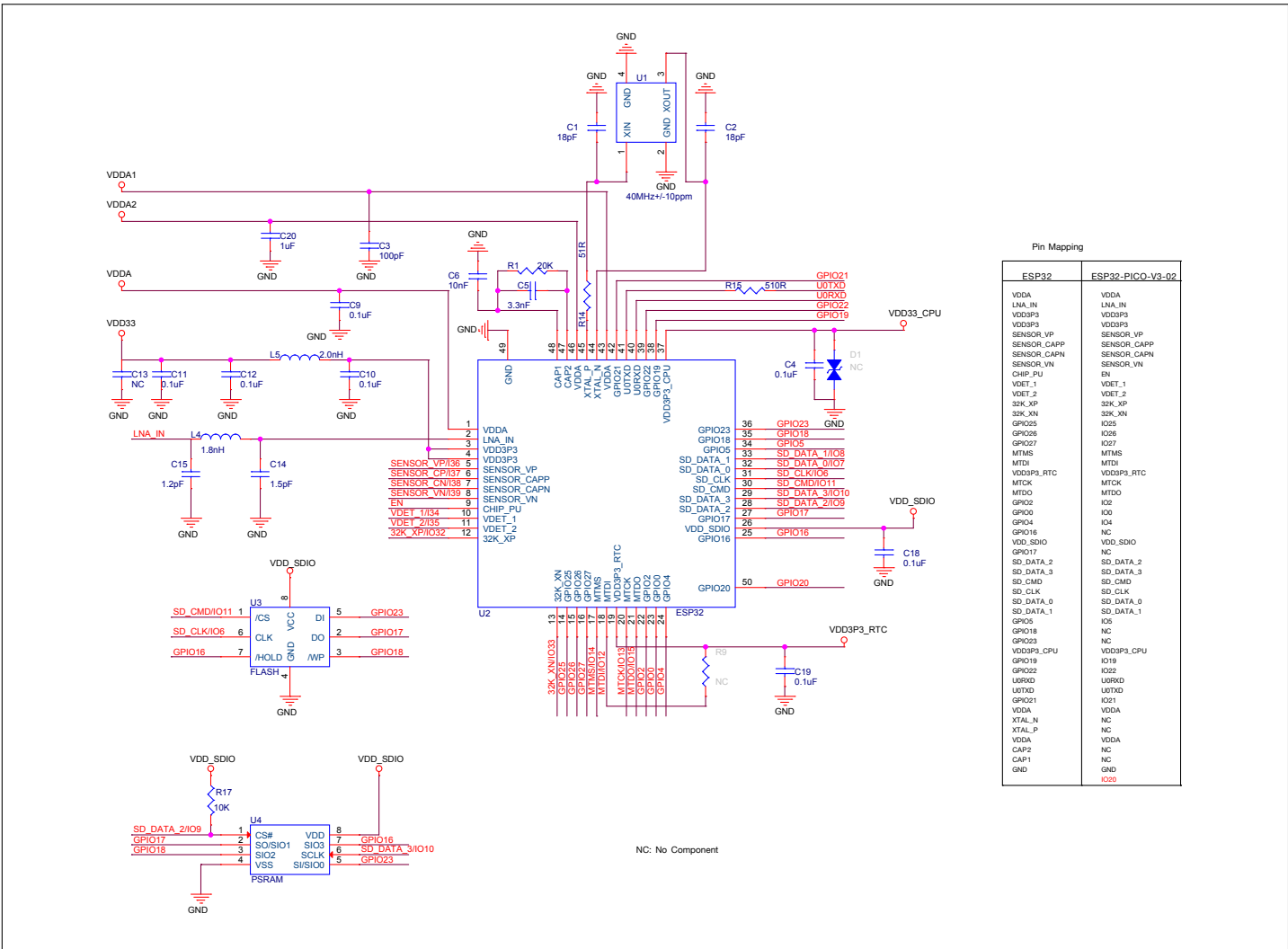
Figure 8: ESP32-PICO-V3-02 Schematics
