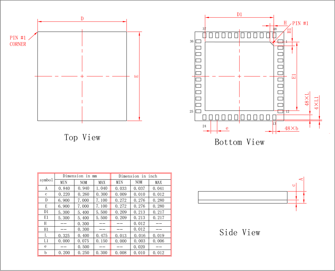
Figure 12: ESP32-PICO-D4 Package
