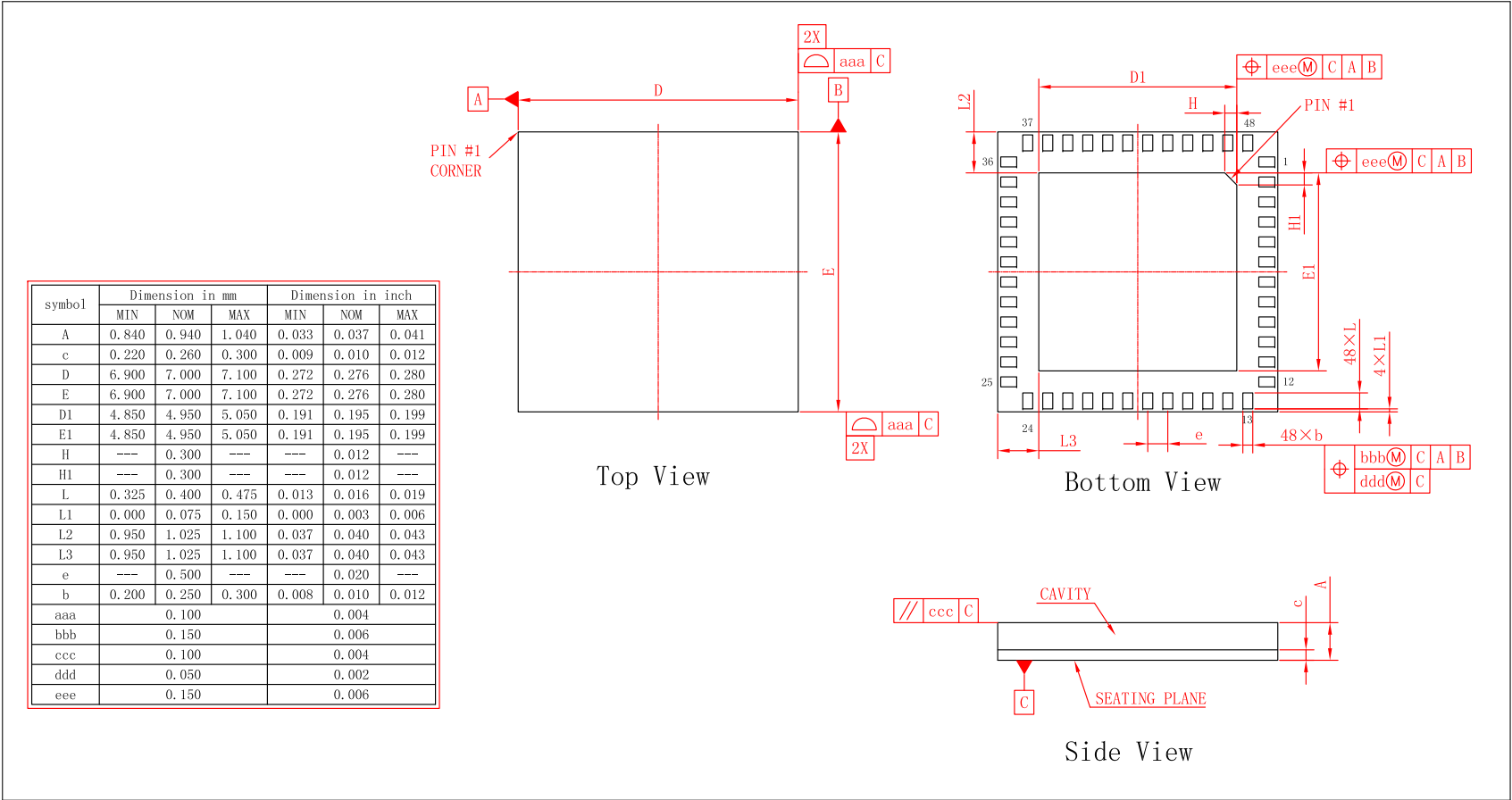
Figure 13: ESP32-PICO-V3 Package
