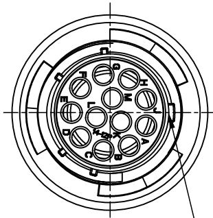
MASTER KEYWAY
