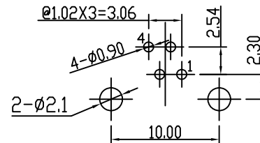
PC BOARD LAYOUT THICKNESS=1.6MM
