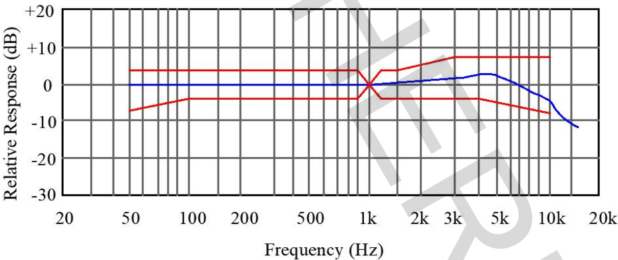
Microphone Response Tolerance Window
