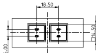
LED arrangement with signal indicator 14.5 x 14.5
