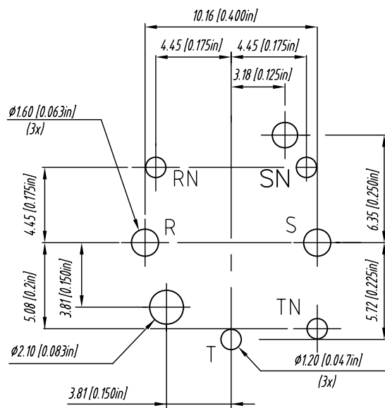
PCB-LAYOUT COMPONENT SIDE TOLERANCE: ±0.05mm [0.002"]
