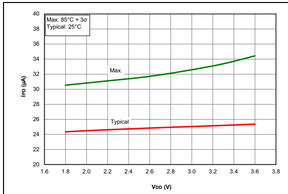
FIGURE 45-50: I_{PO} , Comparator, PIC18LF26/27/45/46/47/55/56/57K42 Only.
