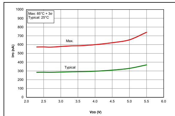
FIGURE 45-53: I_{PO} Base, LP Sleep Mode, PIC18F26/27/45/46/47/55/56/57K42 Only
