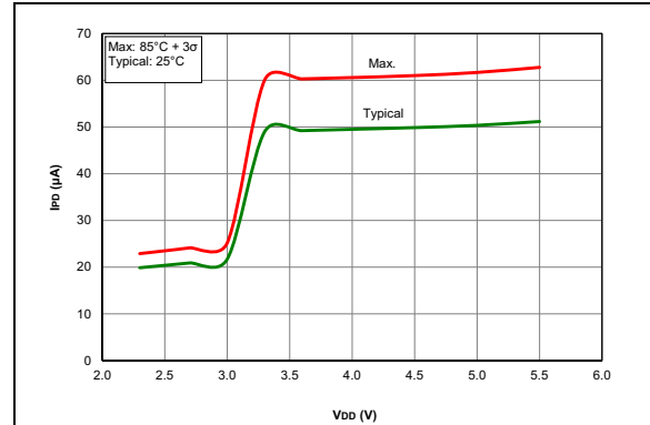
FIGURE 45-52: I_{PO} Base, NP Sleep Mode, PIC18F26/27/45/46/47/55/56/57K42 Only.
