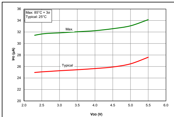
FIGURE 45-51: I_{PO} , Comparator, PIC18F26/27/45/46/47/55/56/57K42 Only.
