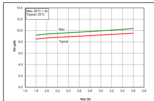
FIGURE 45-54: I_{PO} , High/Low Voltage detect (HLVD), PIC18LF26/27/45/46/47/55/56/57K42 Only.
