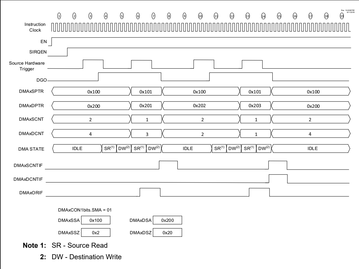
FIGURE 15-9: OVERRUN INTERRUPT
