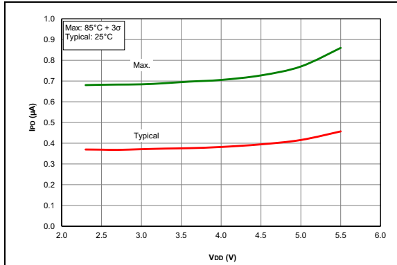
FIGURE 45-49: I_{PO} , Low-Power Brown-Out Reset (LPBOR), PIC18F26/27/45/46/47/55/56/57K42 Only.
