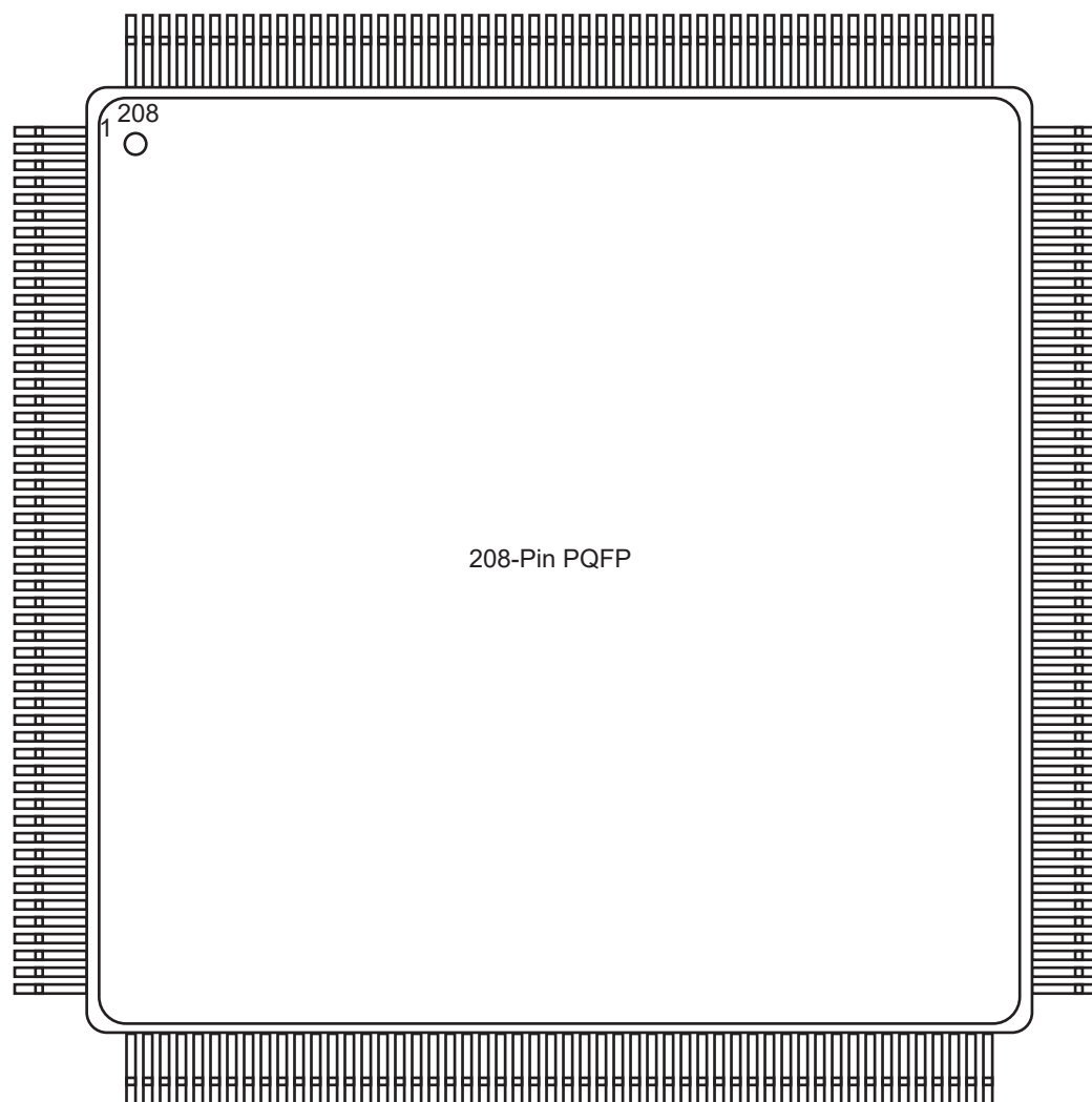
FIGURE 4-6 • PQ208—TOPVIEW
