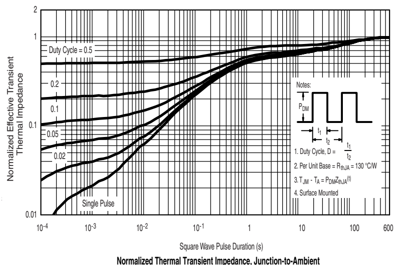
Normalized Thermal Transient Impedance, Junction-to-Ambient
