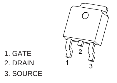
TO-252-2L
