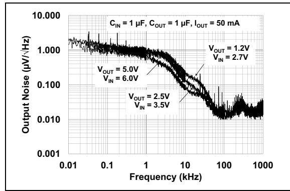
FIGURE 2-29: Output Noise vs. Frequency.
