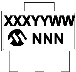
3-Lead SOT-89
