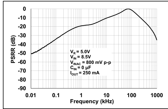
FIGURE 2-28: PSRR vs. Frequency.
