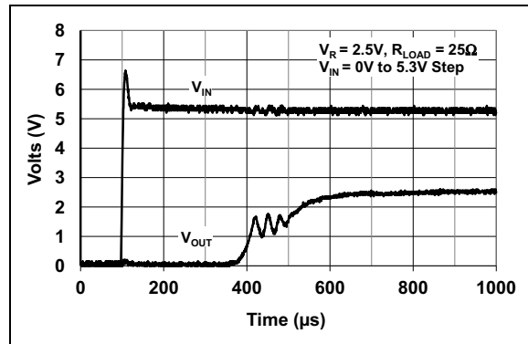
FIGURE 2-30: Power Up Timing.
