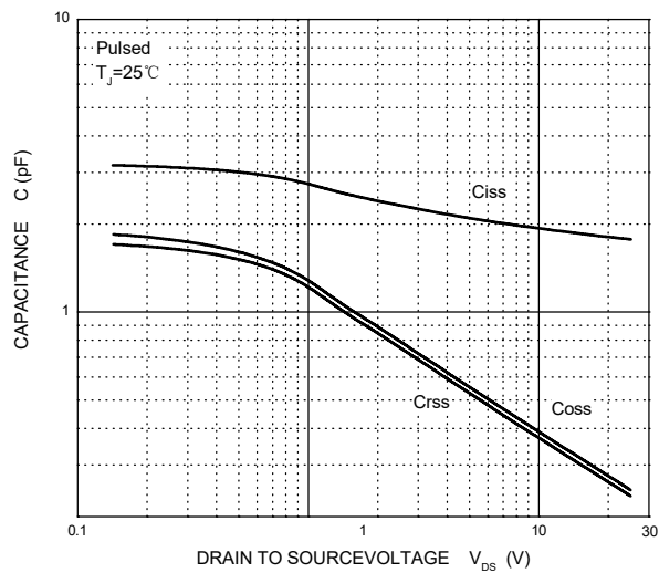
Capacitances
