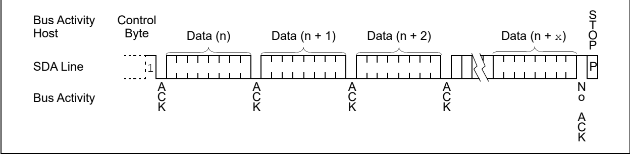
FIGURE 8-3: SEQUENTIAL READ
