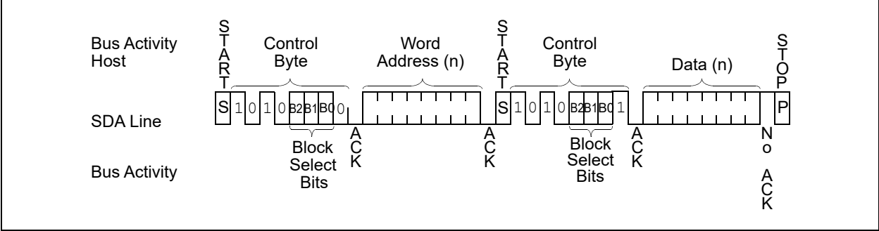
FIGURE 8-2: RANDOM READ
